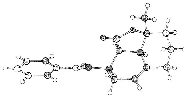
Figure 1. Perspective view of the tricyclic lactone 19 .
